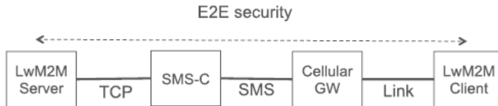
Figure 3: Example of E2E Security over varying Transport
