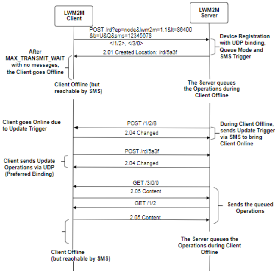
Figure 9: Example of Registration Update Trigger
