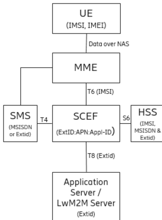
Figure 8: External ID in SCEF
