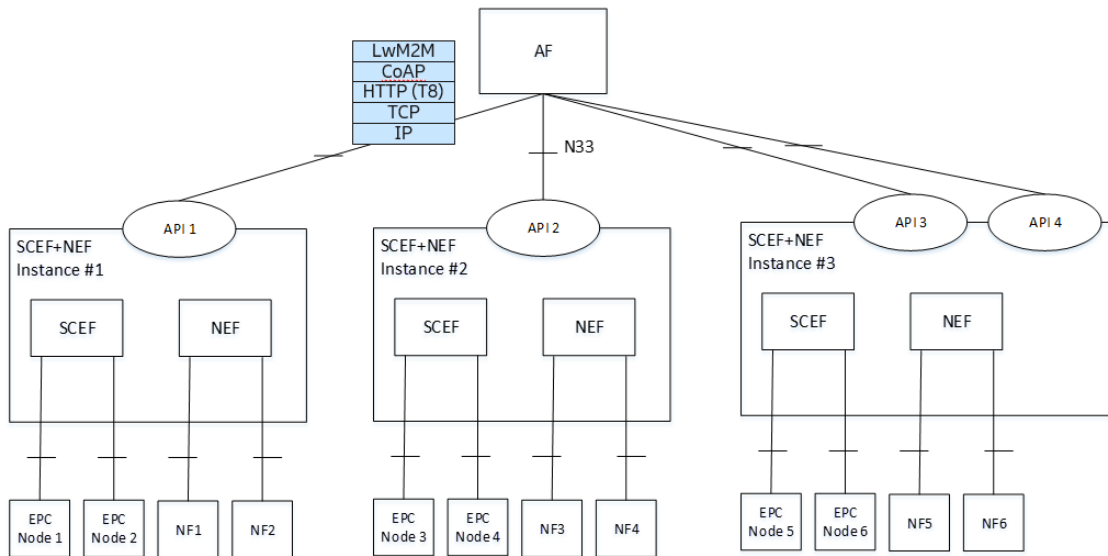
Figure 6: SCEF + NEF Architecture
