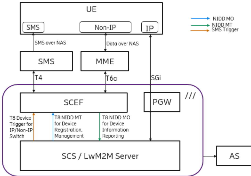
Figure 9: Support for NIDD with LwM2M
