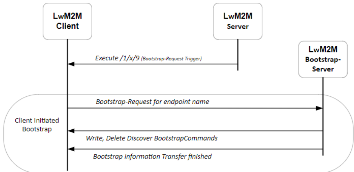
Figure 2: Server Initiated Bootstrap
