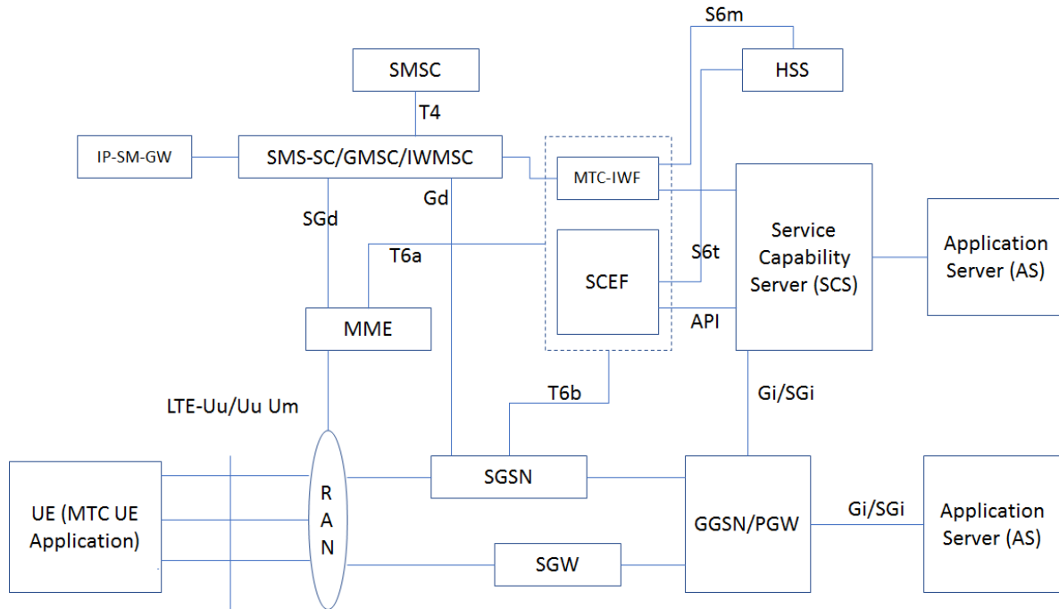
Figure 5: Service Capability Exposure Function
