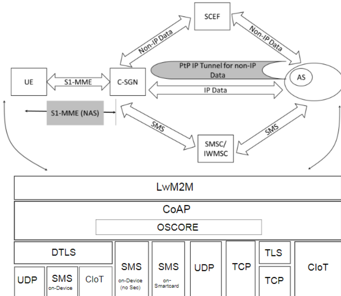
Figure 7: LwM2M over Cellular IoT
