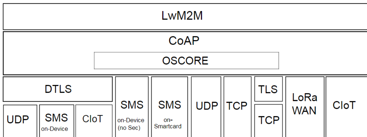
Figure 1: LwM2M 1.1 Protocol Stack
